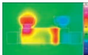
Thermal image without GROHE CoolTouch®
